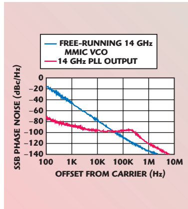
▲ Fig. 7 Measured phase noise .
